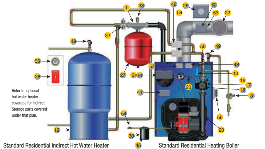
Standard Residential Indirect Hot Water Heater
