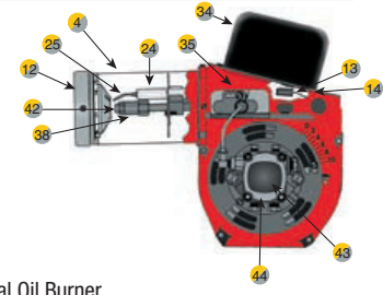
Standard Residential Oil Burner
